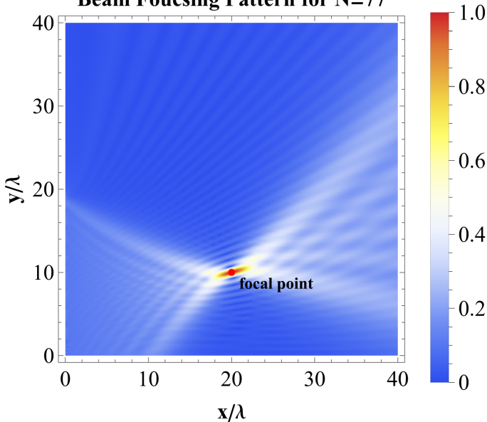
Beam Focusing Pattern for N=77
